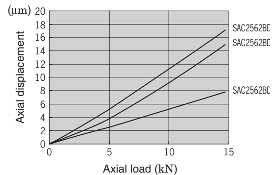
Fig. 5.4 Relationship between axial load and displacement (support bearings for precision ball screws)
