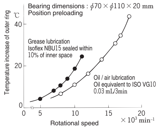
Fig. 8. 5 Comparison of the temperature increase between oil / air lubrication and grease lubrication
