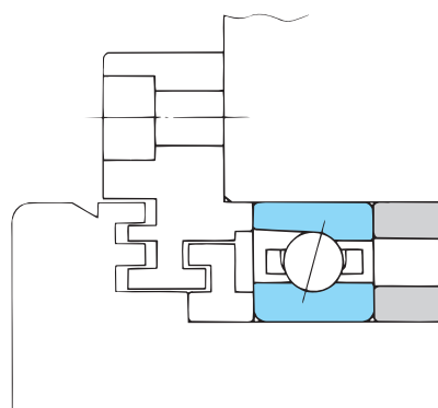
Fig. 8. 3 Example of sealing device for grease lubrication (labyrinth seal)
