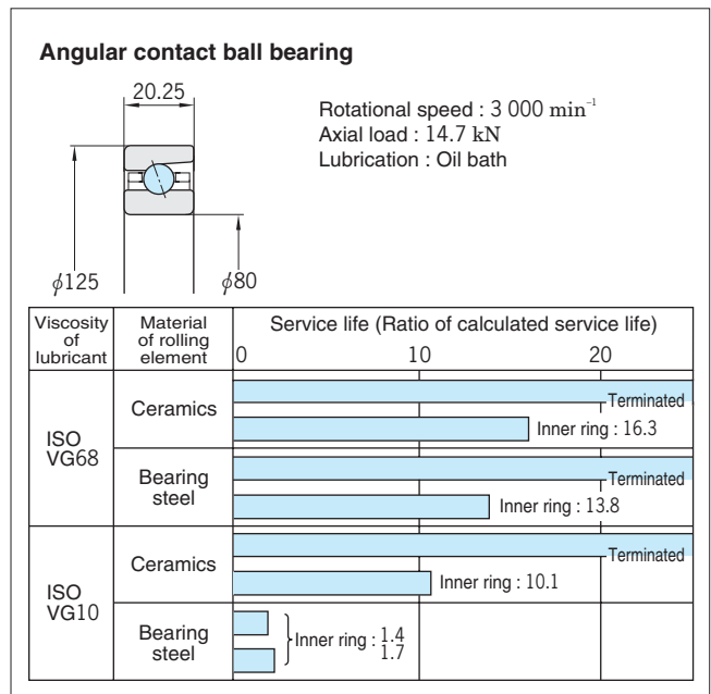
Fig. 11. 11 Life test results of a hybrid ceramic bearing
