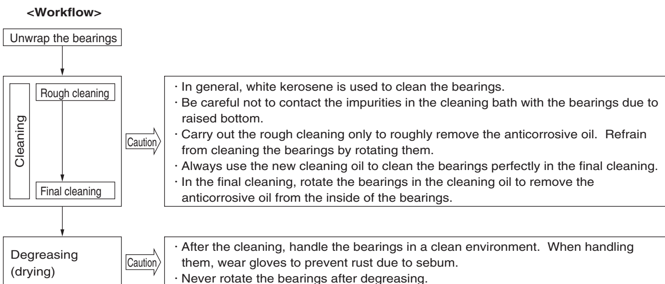
Fig. 1. 5 Cleaning workflow
