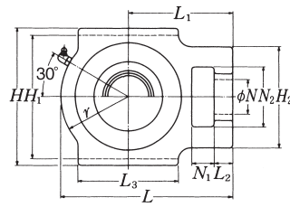
Pressed steel dust cover type Open end Z-UKT...D1 Closed end ZM-UKT...D1
