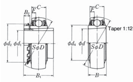
UK2...D1;H, HA, HE, HS
