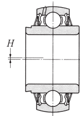
Eccentric locking collar type
