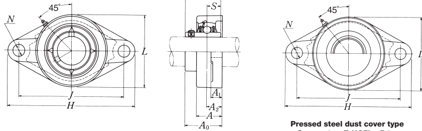
Pressed steel dust cover type Open end Z-UCFL...D1 Closed end ZM-UCFL...D1
