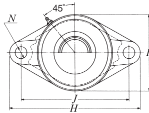
Pressed steel dust cover type Open end Z-UKFL...D1 Closed end ZM-UKFL...D1
