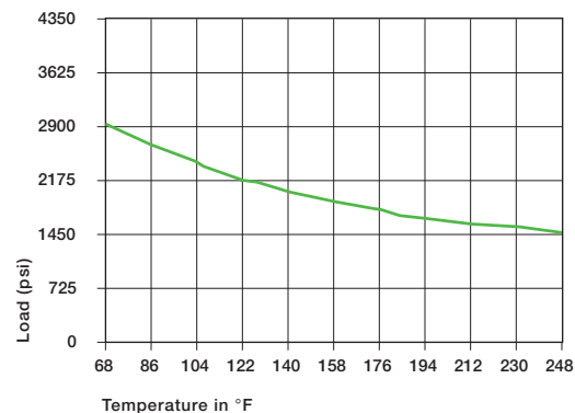
Graph 12.3: Recommended maximum permissible static surface pressure of iglide® A200 as a result of the temperature
