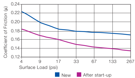
Graph 25.4: Coefficients of friction under load/DryLin® T, v = 29.5 fpm
