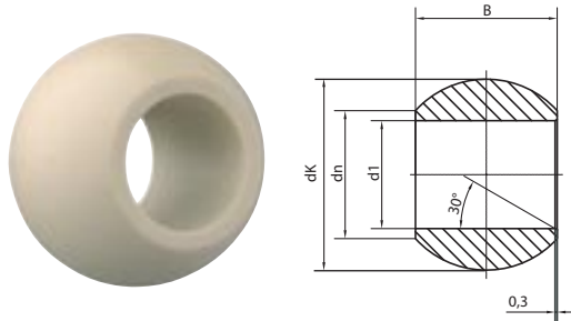
Dimensions (mm) igubal® Spherical Bearings JKM
