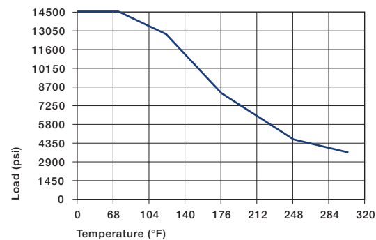
Graph 8.3: Recommended maximum static surface pressure of iglide® Q as a result of the temperature
