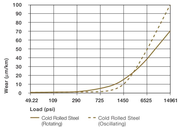
Graph 7.9: Wear for oscillating and rotating applications with shaft material Cold Rolled Steel, as a result of the load
