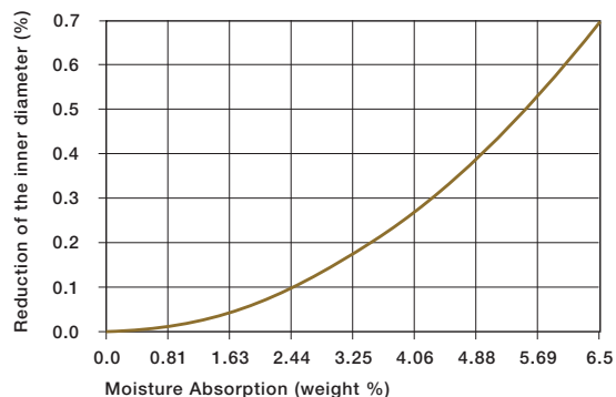
Graph 7.10: Effect of moisture absorption on iglide® L280 plain bearings
