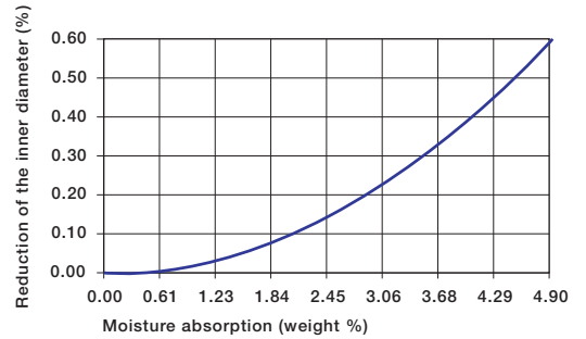
Graph 8.11: Effect of moisture absorption on iglide® Q plain bearings
