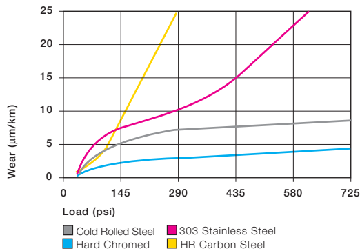
Graph 8.8: Wear with different shaft materials for rotating applications
