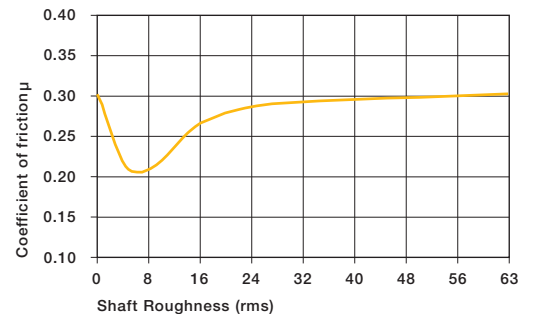
Graph 9.6: Coefficients of friction of iglide® P as a result of the shaft surface (shaft Cold Rolled Steel)
