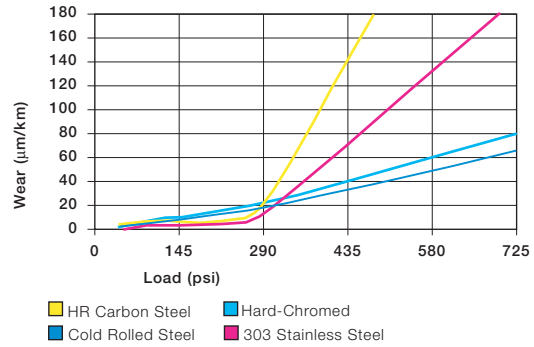
Graph 13.9: Wear of iglide® T500 with different shaft materials in rotational operation
