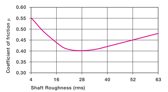
Graph 2.6: Coefficient of friction for iglide® M250 as a result of the shaft surface (shaft Cold Rolled Steel)
