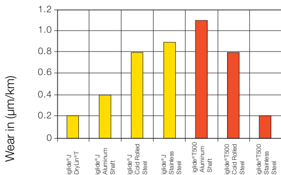
Graph 25.8: Wear in µm/km for different sliding partners, p = 145 psi
