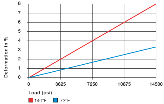
Graph 13.2: Deformation under load and temperature
