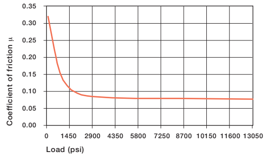
Graph 13.6: Coefficient of friction for iglide® T500 as a result of the load, v = 1.97 fpm
