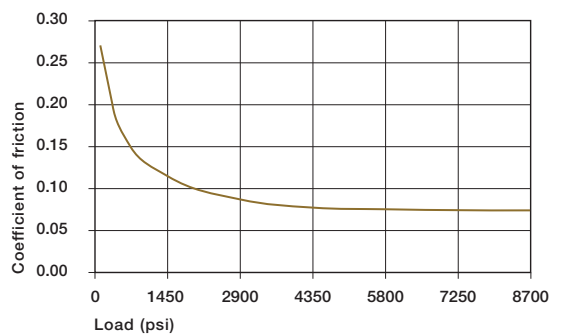
Graph 7.5: Coefficient of friction of iglide® L280 as a result of the load, v = 1.97 fpm
