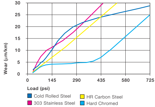
Graph 12.8: Wear of iglide® A200 with different shaft materials in rotational applications
