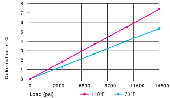
Graph 15.2: Deformation under load and temperature
