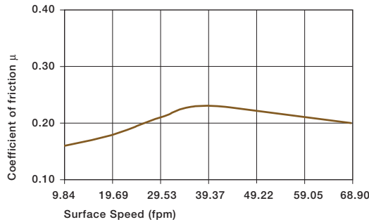
Graph 15.5: Coefficients of friction of iglide® Z as a result of the running speed; p = 108 psi
