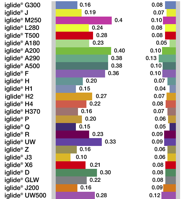
Frictional values of iglide® materials under different loads
