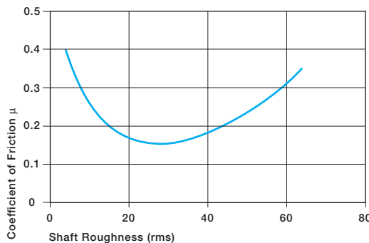
Graph 6.6: Coefficient of friction as result of the shaft surface (Shaft - Cold Rolled Steel)
