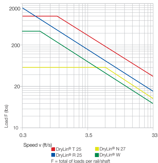
Graph 25.1: F x V values of comparable DryLin® systems
