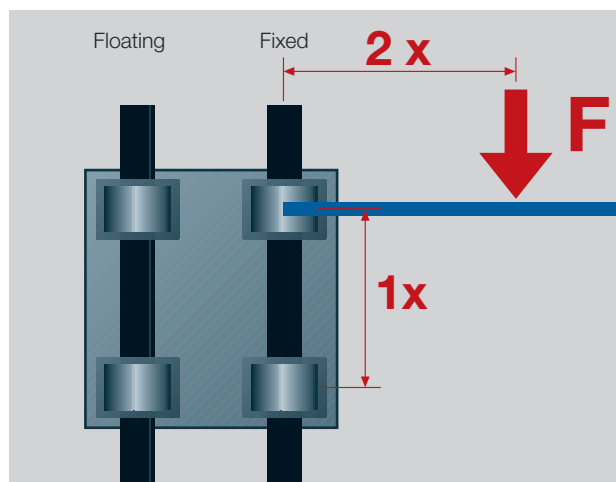
The 2:1 Rule
