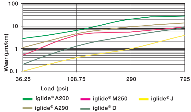
Wear of iglide® plain bearings for small loads, shaft: Cold Rolled Steel, v=19.7 fpm
