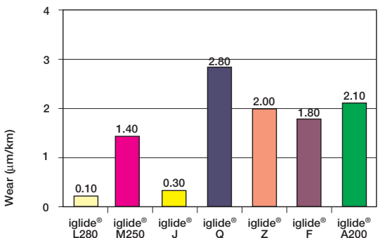
Wear with shaft X90, p = 108.75 psi, v = 98 fpm, shaft finish = 8 rms
