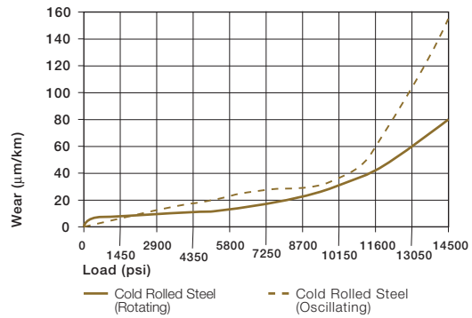
Graph 15.10: Wear for oscillating and rotating applications with Cold Rolled Steel shafts
