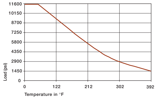
Graph 10.3: Recommended permissible maximum static surface pressure of iglide® H370 as a result of the temperature
