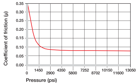
Graph 13.5: Coefficient of friction as a function of the pressure, v = (0.01 m/s) fpm
