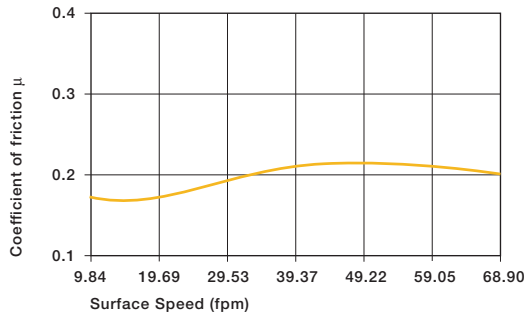
Graph 9.4: Coefficients of friction of iglide® P as a result of the surface speed; p = 108 psi
