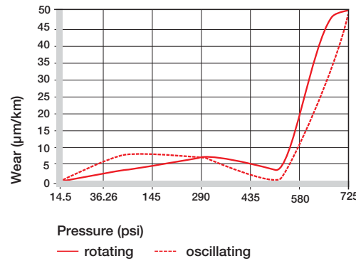
Graph 13.9: Wear for oscillating and rotating applications with shaft materials c53 hardened and ground steel, as a function of the pressure
