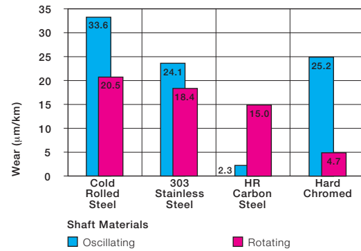
Graph 12.9: Wear with different shaft materials, oscillating and rotating movement p = 290 psi
