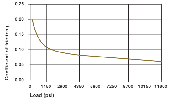
Graph 15.6: Coefficients of friction of iglide® Z as a result of the load, v = 1.97 fpm
