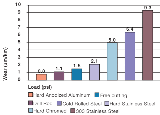
Graph 12.7: Wear of iglide® A200, rotating applications with different shaft materials, p=108 psi, v=98 fpm
