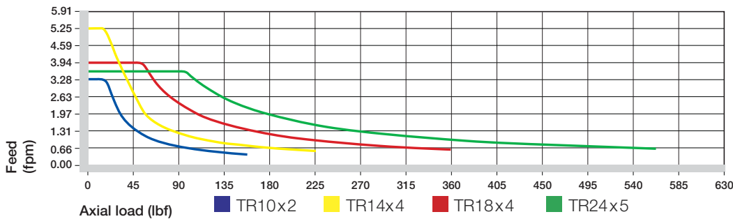
Maximum Feed (fpm)
