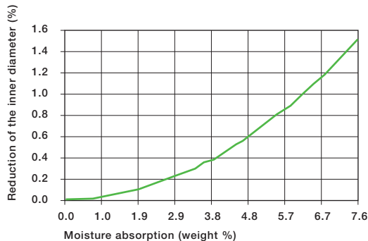
Graph 12.10: Effect of moisture absorption on iglide® A200 plain bearings
