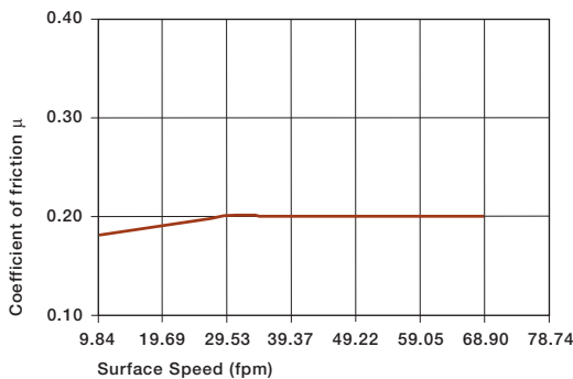
Graph 10.5: Coefficients of friction for iglide® H370 as a result of the surface speed; p = 108 psi
