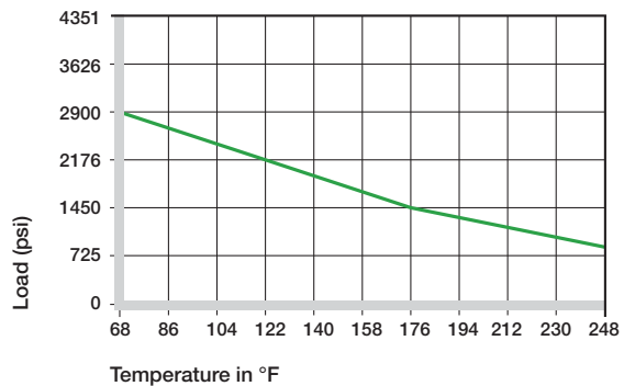
Graph 12.3: Recommended maximum permissible static surface pressure of iglide® A200 as a result of the temperature
