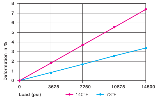
Graph 10.2: Deformation under load and temperature
