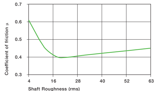
Graph 12.6: Coefficients of friction of iglide® A200 as a function of the shaft surface (shaft Cold Rolled Steel)
