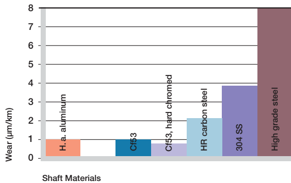
Graph 11.7: Wear of iglide® A180, rotating applications with different shaft materials, p=108 psi, v=98 fpm
