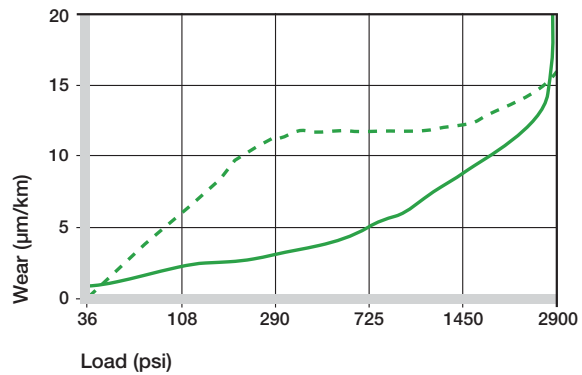
Graph 11.8: Wear of iglide® A180 with different shaft materials in rotational applications
