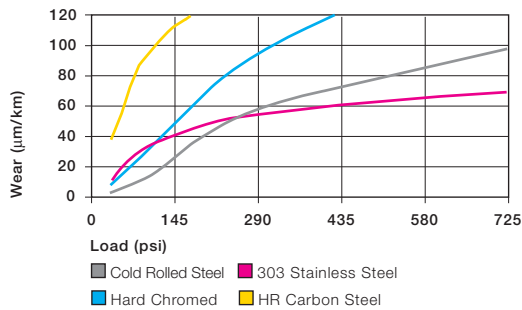
Graph 15.9: Wear of iglide® Z with different shaft materials in rotating applications
