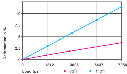
Graph 20.2: Deformation under load and temperature
