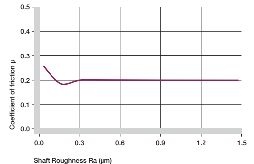
Graph 3.6: Coefficient of friction for iglide® R as a result of the shaft surface (shaft Cold Rolled Steel)
