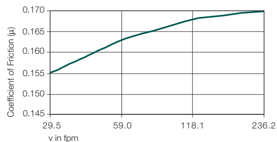
Graph 25.7: Coefficient of friction as a result of the speed/DryLin® T, p = 67 psi
