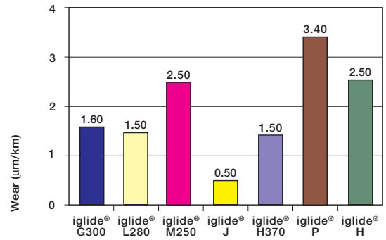
Wear with shaft HR Carbon Steel, p = 108.75 \text{ psi} , v = 98 \text{ fpm} , shaft finish = 8 rms
