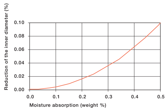
Graph 13.11: Effect of moisture absorption on iglide® T500 plain bearings
