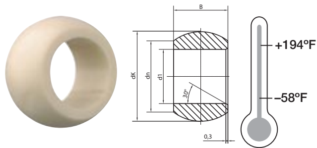
Dimensions (mm) igubal® Spherical Bearings JEM
