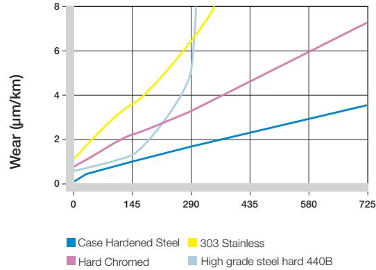
Graph 3.8: Wear of iglide® R with different shaft materials in rotational operation
