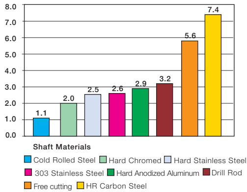
Graph 15.8: Wear of iglide® Z rotating applications with different shaft materials, p=108 psi, v=98 fpm
