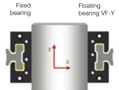
Horizontal mounting version with floating bearing in the Y-direction and lateral mounting carriage
