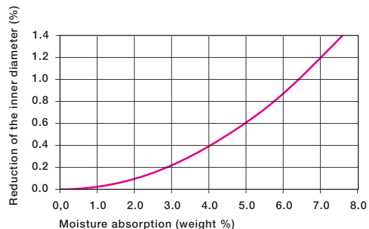
Graph 2.10: Effect of moisture absorption on iglide® M250 plain bearings
