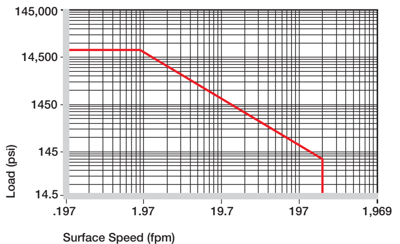
Graph 13.1: Permissible p x v value for iglide® M250 running dry against a steel shaft, at 68°F
