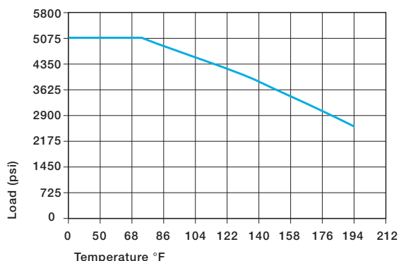
Graph 20.3: Recommended maximum permissible static surface pressure of iglide® J as a result of the temperature
