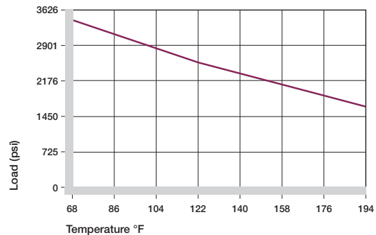
Graph 3.3: Recommended maximum permissible static surface pressure of iglide® R as a result of the temperature
