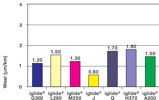
Wear with a machining steel shaft, p=108.75 psi, v = 98 fpm, shaft finish = 8 rms
