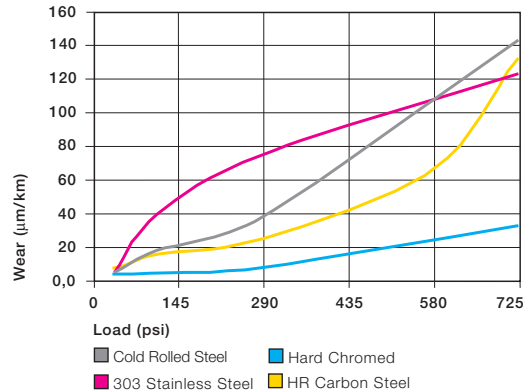
Graph 10.9: Wear of iglide® H370 with different shaft materials in rotating applications
