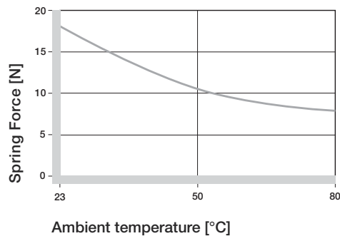
Effect of ambient temperature on the spring force
