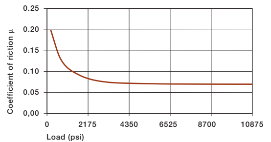
Graph 10.6: Coefficients of friction for iglide® H370 as a result of the load, v = 1.97 fpm
