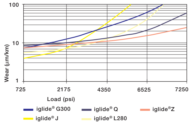
Wear of iglide® plain bearings for medium and high loads, shaft: Cold Rolled Steel, v=19.7 fpm
