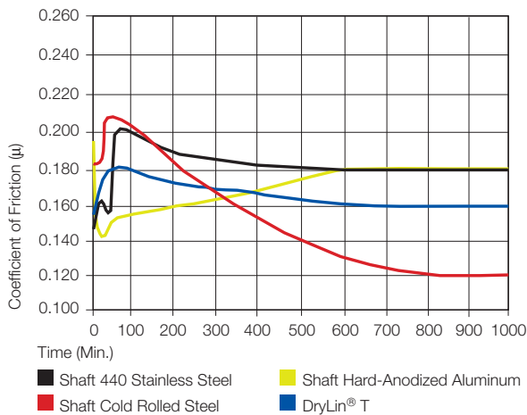
Graph 25.2: DryLin® long-term progression of the coefficient of friction, p = 130 psi, v = 29.5 fpm
