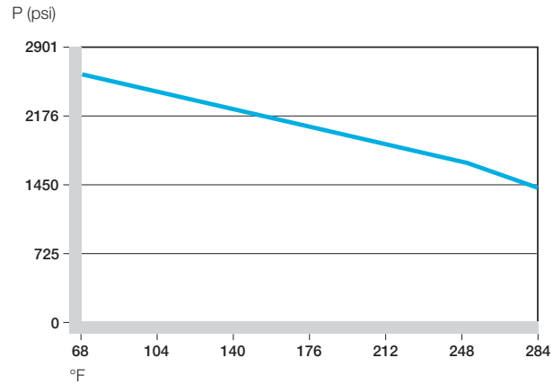
Graph 19.1: Permissible static surface pressure as a result of the operating temperature for clip bearings made of iglide® M250
