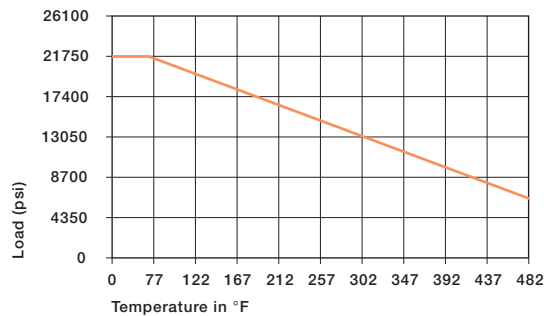
Graph 13.3: Recommended maximum permissible static surface pressure of iglide® T500 as a result of temperature
