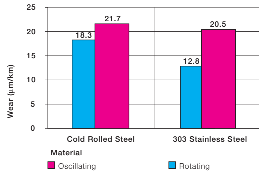
Graph 13.10: Wear for oscillating and rotating applications with different shaft materials p = 290 psi
