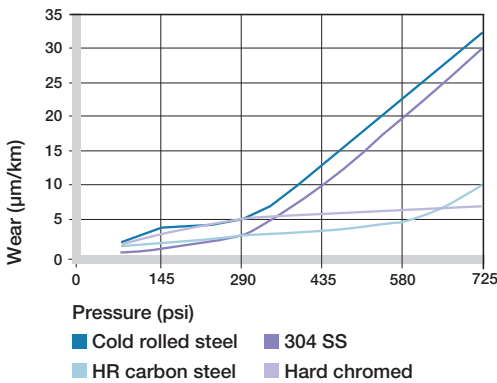
Graph 13.8: Wear with different shaft materials in rotational operation, as a function of the pressure
