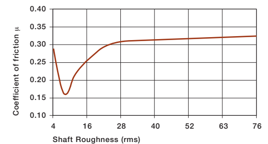
Graph 10.7: Coefficient of friction of iglide® H370 as a result of the shaft surface (shaft Cold Rolled Steel)
