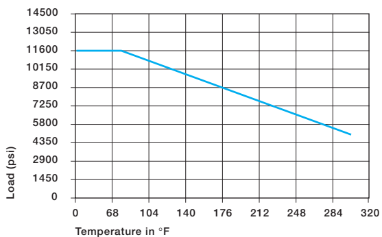
Graph 6.3: Recommended maximum permissible static surface pressure of iglide® G300 as a result of temperature
