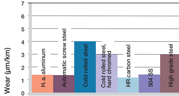
Graph 13.7: Wear rotating with different shaft materials, p = 145 \text{ psi} , v = 59 \text{ fpm}
