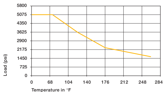
Graph 9.3: Recommended maximum permissible static surface pressure of iglide® P as a result of the temperature
