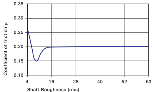
Graph 8.6: Coefficient of friction as a result of the shaft surface
