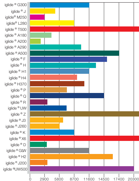
Permissible average static surface pressure at 68°F
