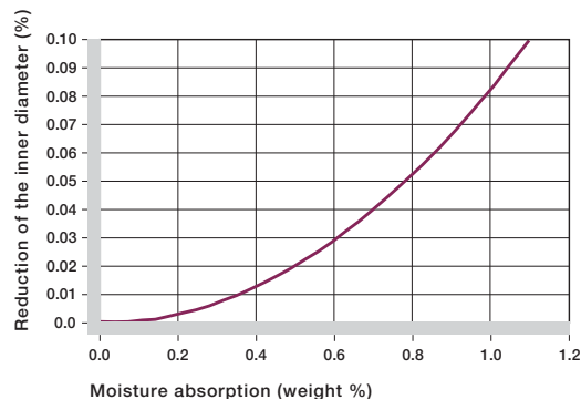
Graph 3.10: Effect of moisture absorption on iglide® R plain bearings
