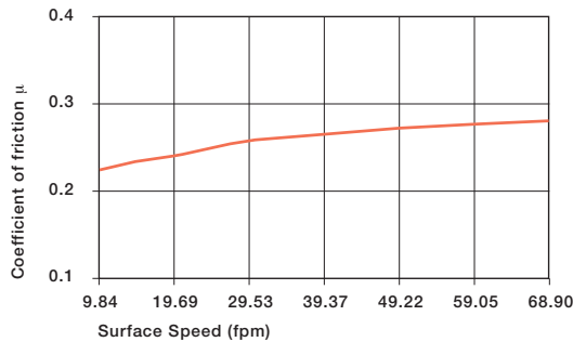
Graph 13.5: Coefficient of friction for iglide® T500 as a result of the surface speed; p = 108 psi, shaft Cold Rolled Steel
