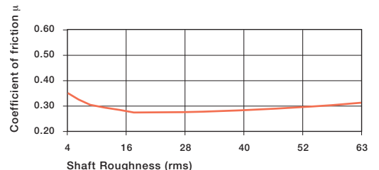
Graph 13.7: Coefficients of friction as a function of the shaft surface (shaft Cold Rolled Steel)
