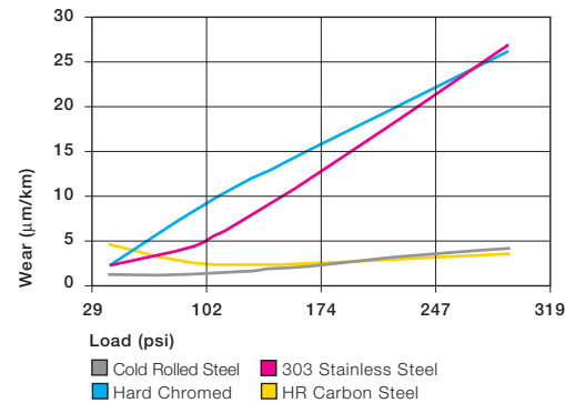
Graph 9.8: Wear of iglide® P with different shaft materials in rotating applications
