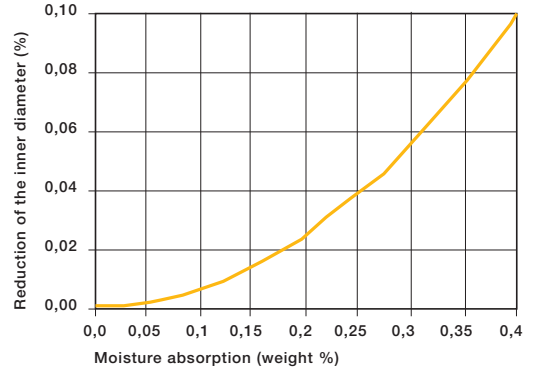
Graph 9.11: Effect of moisture absorption on iglide® P plain bearings
