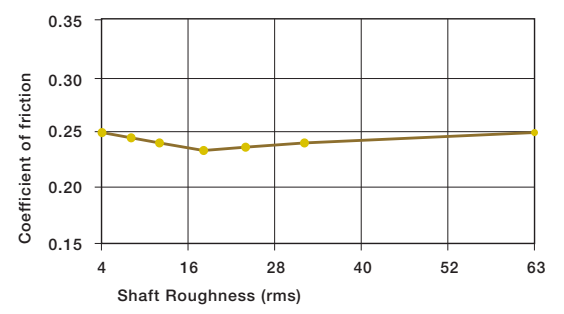
Graph 7.6: Coefficients of friction for iglide® L280 as a result of the shaft surface (shaft Cold Rolled Steel)
