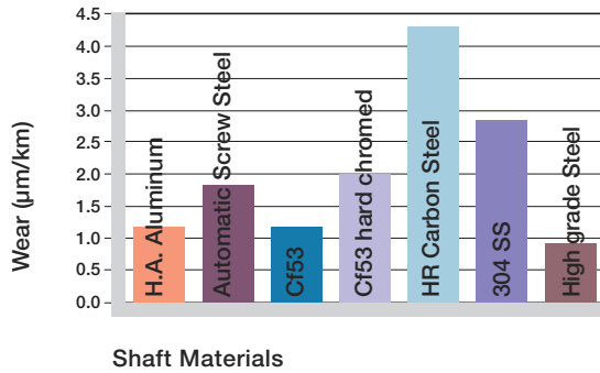
Graph 3.7: Wear for iglide® R, rotating with different shaft materials, p = 108 psi, v = 98 fpm
