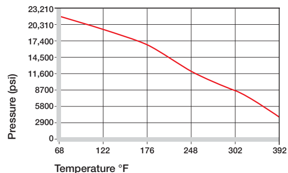
Graph 13.3: Recommended maximum permissible static surface pressure of iglide® X6 as a result of temperature (21,760 psi at +68°F)
