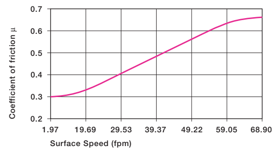
Graph 2.4: Coefficient of friction of iglide® M250 as a result of the surface speed; p = 108 psi
