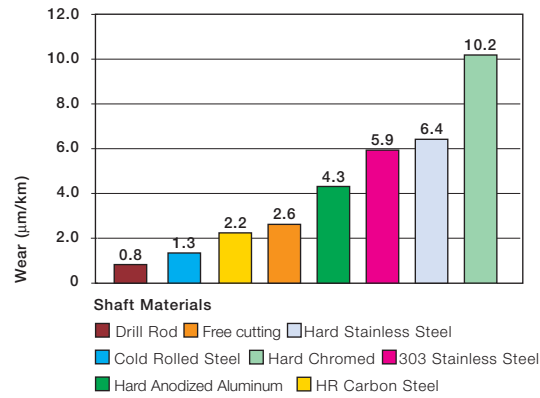
Graph 9.7: Wear of iglide® P with different shaft materials in rotating applications, p=108 psi, v=98 fpm
