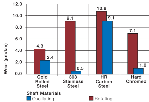
Graph 15.11: Wear for oscillating and rotating applications with different shaft materials, load p = 290 psi
