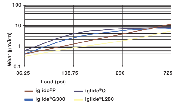
Wear of iglide® plain bearings under low loads
