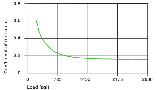
Graph 12.5: Coefficients of friction of iglide® A200 as a function of the load, v = 0.01 m/s
