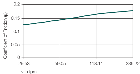
Graph 25.6: Coefficient of friction as a result of the speed/DryLin® R, p = 130 psi
