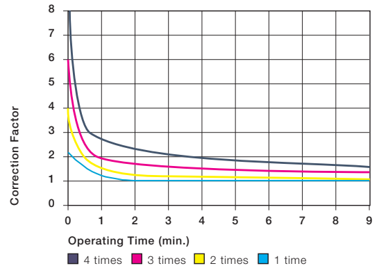
Correction factor for p x v-value
