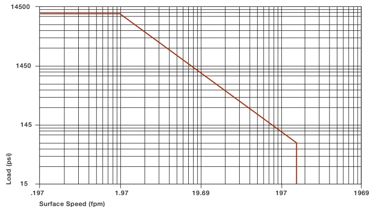
Graph 10.1: Permissible p x v value for iglide® H370 running dry against a steel shaft, at 68°F
