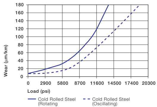
Graph 8.9: Wear for oscillating and rotating applications with a Cold Rolled Steel shaft
