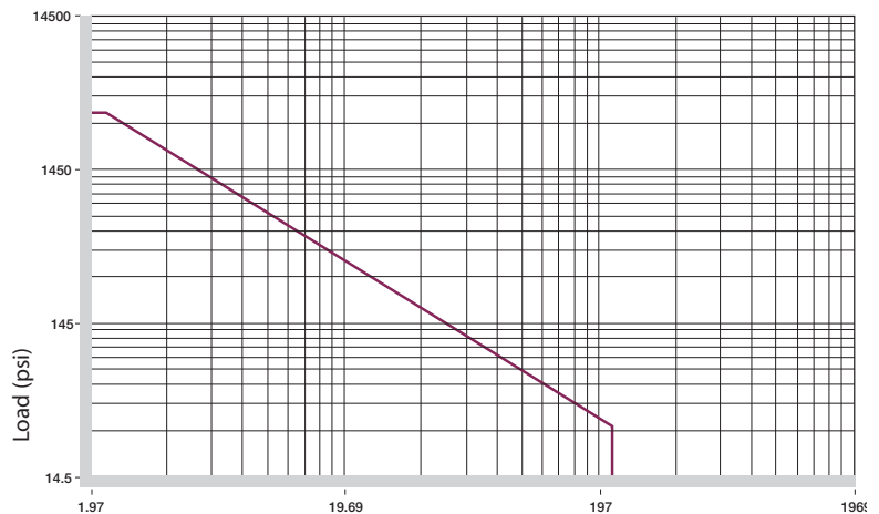
Graph 3.1: Permissible p x v value for iglide® R running dry against a steel shaft, at 68°F
