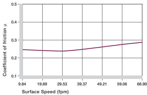
Graph 3.4: Coefficient of friction of iglide® R as a result of the surface speed; p = 108 psi
