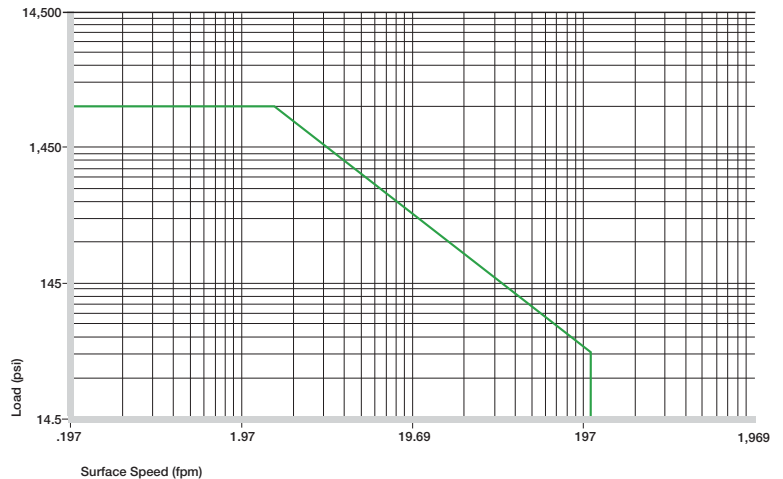
Graph 12.1: Permissible p x v values for iglide® A200 running dry against a steel shaft, at 68°F
