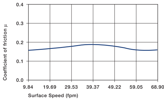
Graph 8.4: Coefficient of friction as a result of the surface speed; load = 108 psi constant
