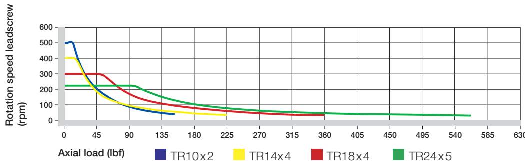
Maximum permissible rotation speed leadscrew (rpm)
