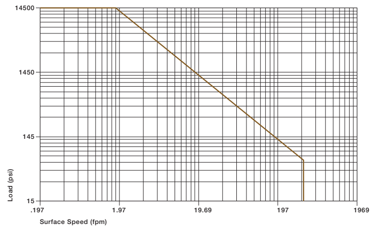
Graph 15.1: Permissible p x v values for iglide® Z running dry against a steel shaft, at 68°F
