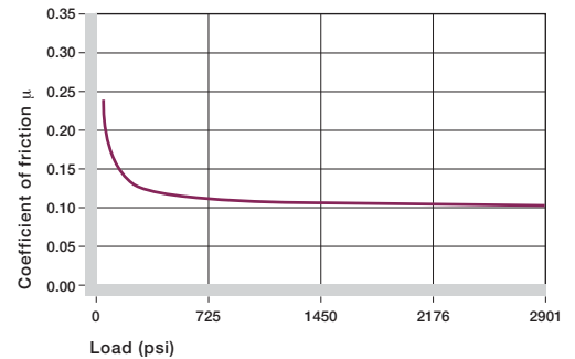
Graph 3.5: Coefficient of friction of iglide® R as a result of the load, v = 1.97 fpm
