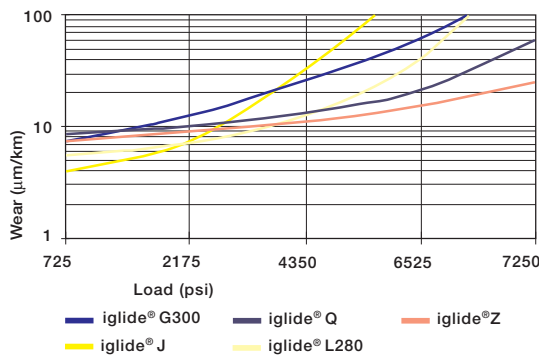
Wear of iglide® plain bearings under medium and high loads
