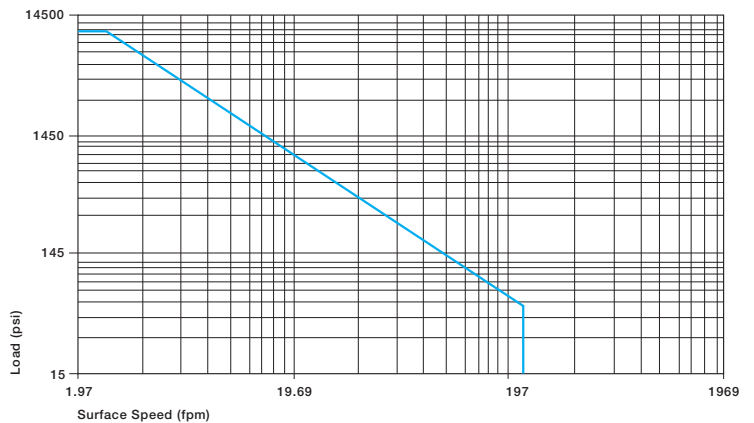
Graph 6.1: Permissible p x v - values for iglide® G300 running dry against a steel shaft, at 68°F
