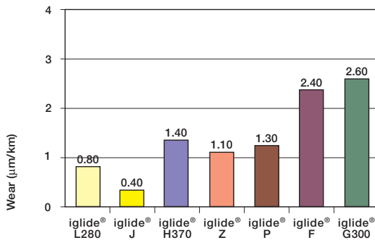
Wear with shaft Cold Rolled Steel, p = 108.75 \text{ psi} , v = 98 \text{ fpm} , shaft finish = 8 rms
