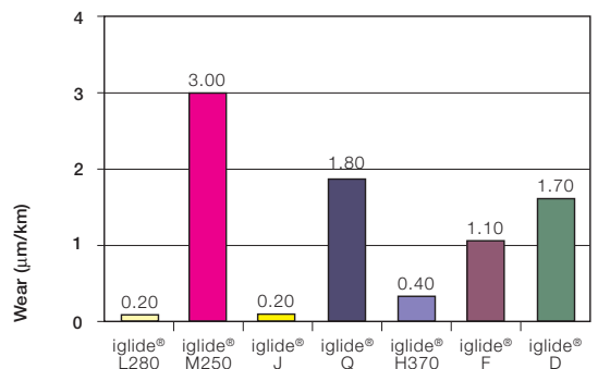
Wear with hard-chromed shaft, p = 108.75 \text{ psi} , v = 98 \text{ fpm} , shaft finish = 8 rms
