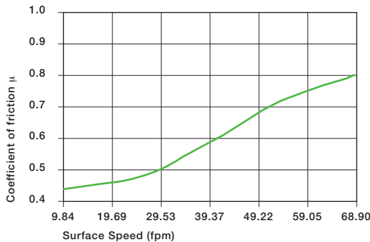
Graph 12.4: Coefficients of friction of iglide® A200 as a function of the running speed; p = 108 psi
