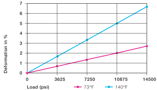
Graph 8.2: Deformation under load and temperature
