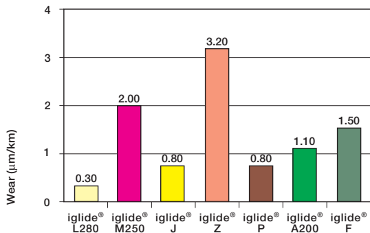
Wear with a silver steel shaft, p=108.75 psi, v=98 fpm, shaft finish = 8 rms
