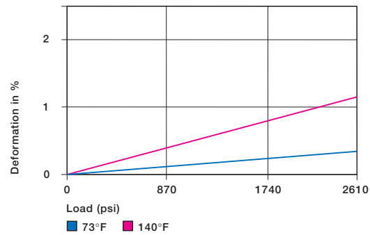
Graph 12.2: Deformation under load and temperature
