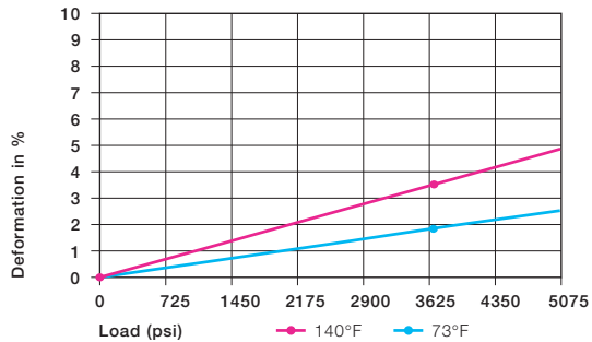
Graph 9.2: Deformation under load and temperature
