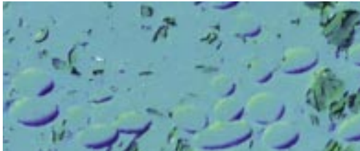
Base plastics with fibers and solid lubricants, magnified 200 times, dyed
