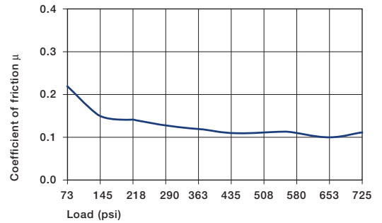
Graph 8.5: Coefficient of friction as a result of the load, v = 1.97 fpm
