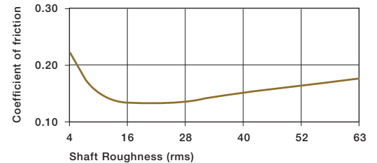
Graph 15.7: Coefficients of friction of iglide® Z as a result of the shaft surface (shaft Cold Rolled Steel)
