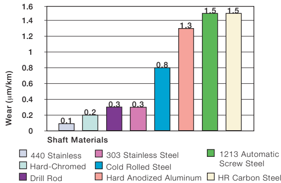
Graph 7.7: Wear of iglide® L280 with different shaft materials (p = 108 psi)
