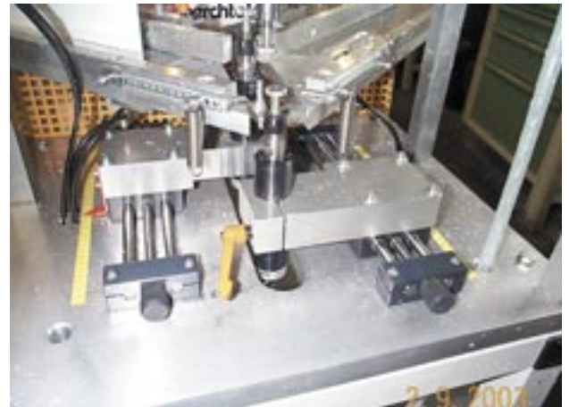
Lead screw table used to position milling heads in aluminum window manufacturing
