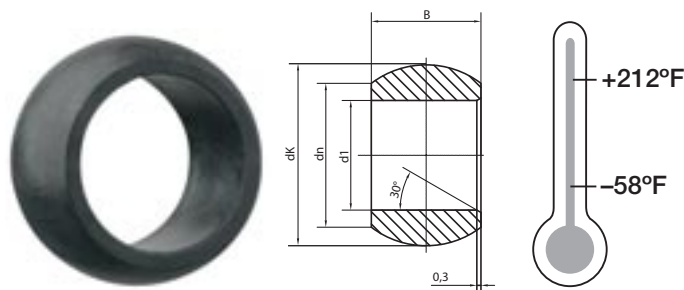
Dimensions (mm) igubal® Spherical Bearings UWEM
