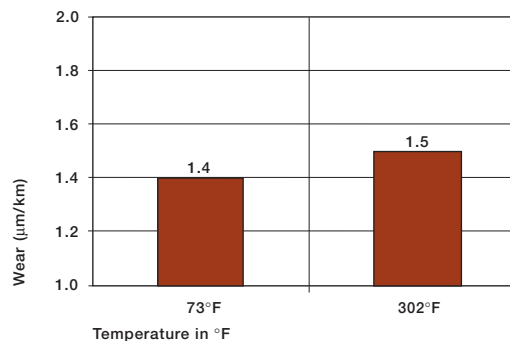
Graph 10.4 : Wear as a result of the temperature; rotation with p = 108 psi and v = 98 fpm
