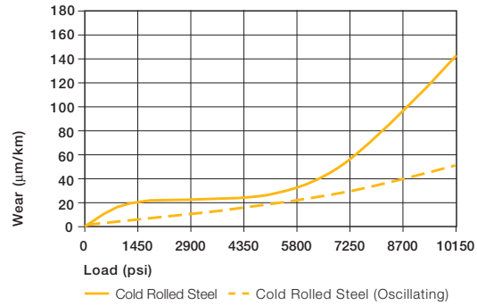
Graph 9.9: Wear with the Cold Rolled Steel shaft in oscillating and rotating applications
