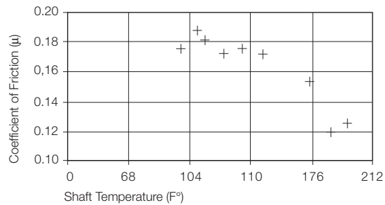
Graph 25.5: Coefficients of friction as a result of the temperature iglide® J versus Aluminum hc, v = 59 fpm, p = 130 psi
