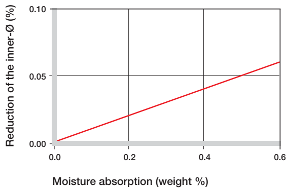
Graph 13.10: Effect of moisture absorption on iglide® X6 plain bearings
