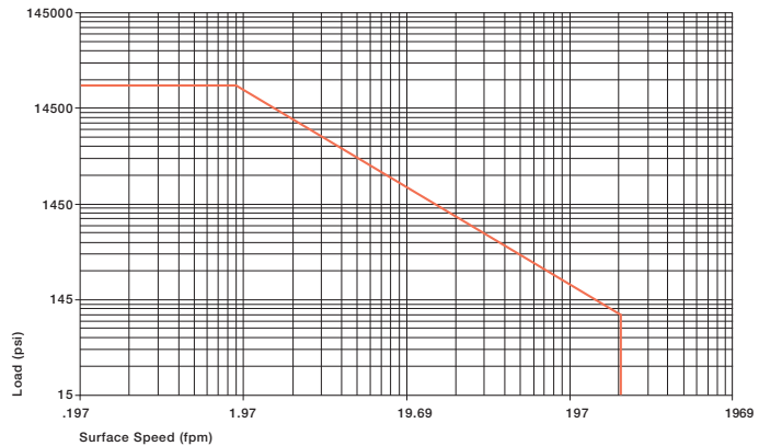
Graph. 13.1: Permissible p x v values for iglide® T500 running dry against a steel shaft, at 68°F
