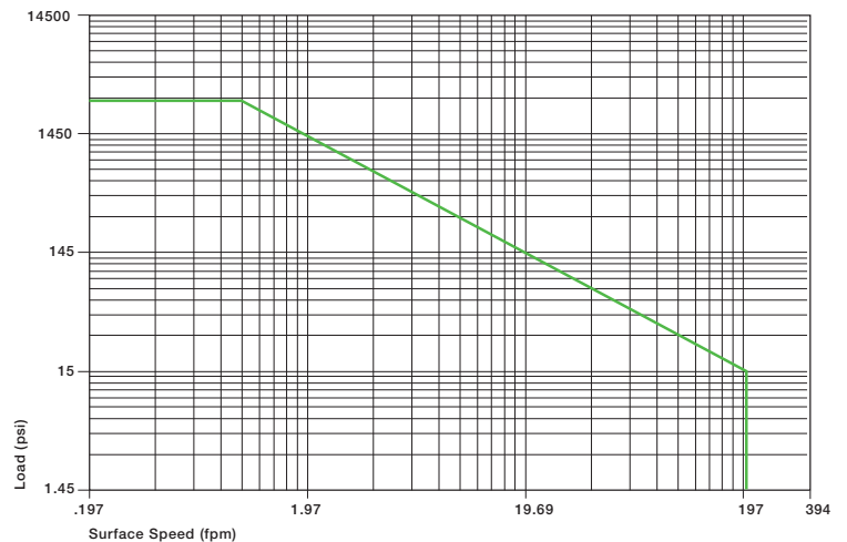
Graph 12.1: Permissible p x v values for iglide® A200 running dry against a steel shaft, at 68°F
