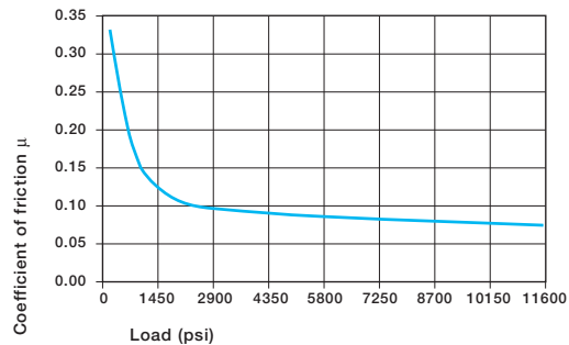
Graph 6.5: Coefficient of friction of iglide® G300 as a result of the load
