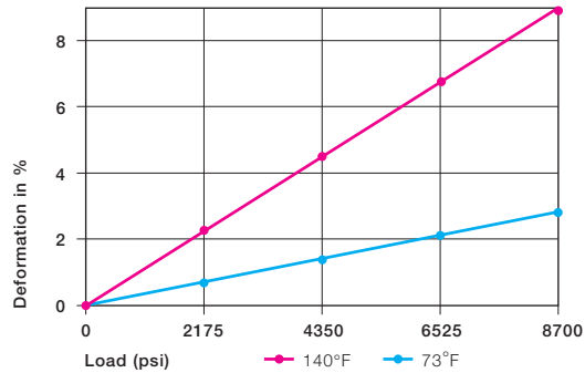
Graph 7.2: Deformation under load and temperature
