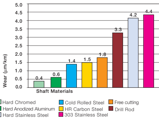
Graph 10.8: Wear of iglide® H370, rotating application with different shaft materials, p=108 psi, v=98 fpm
