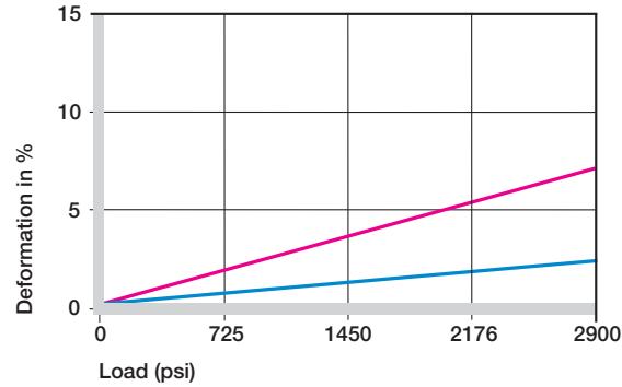
Graph 12.2: Deformation under load and temperature
