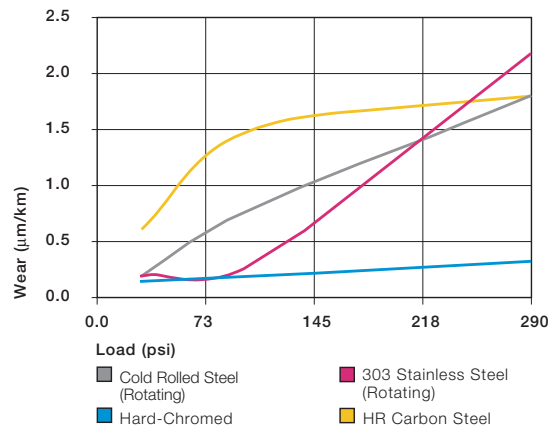
Graph 7.8: Wear with different shaft materials in rotational operation, as a result of the load
