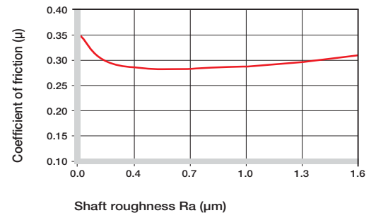
Graph 13.6: Coefficients of friction as a function of the shaft surface (cf53 hardened and ground steel)
