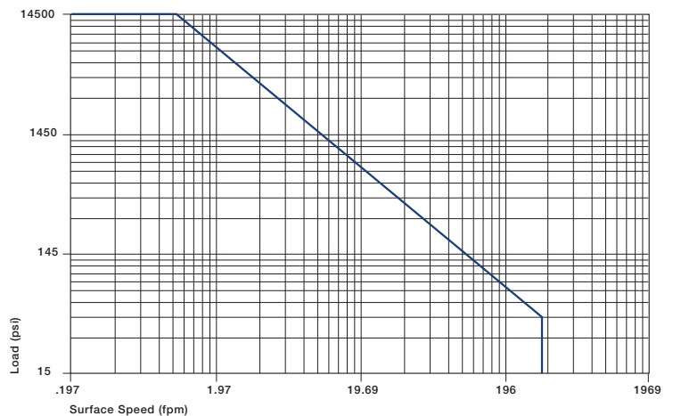
Graph 8.1: Permissible p x v value for iglide® Q running dry against a steel shaft, at 68°F
