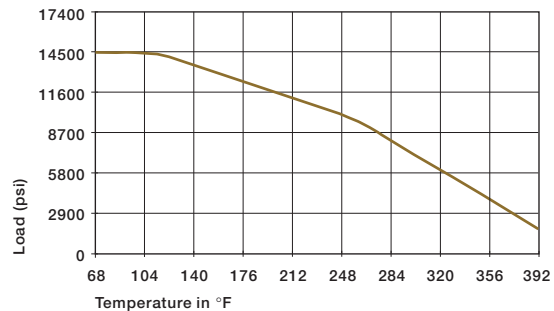
Graph 15.3: Recommended maximum permissible static surface pressure of iglide® Z as a result of the temperature
