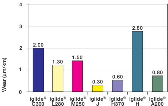
Wear with an aluminum shaft, p=108.75 psi, v=98 fpm, shaft finish = 8 rms
