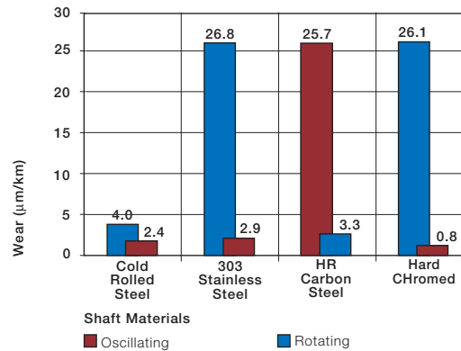
Graph 9.10: Wear with different shaft materials in oscillating and rotating applications p = 290 psi
