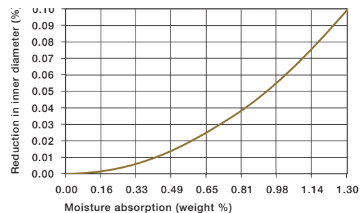
Graph 4.10: Effect of moisture absorption on iglide® J plain bearings
