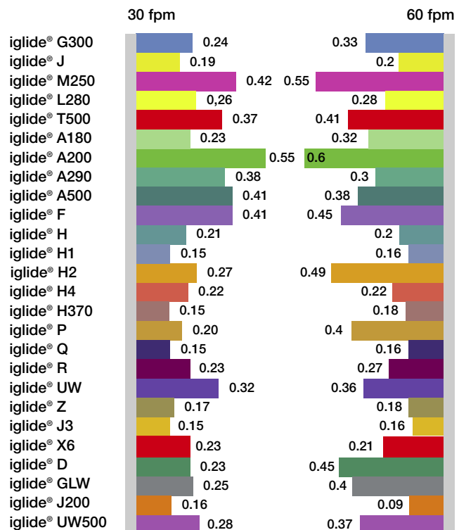
Coefficients of friction of iglide® materials for different surface speeds
