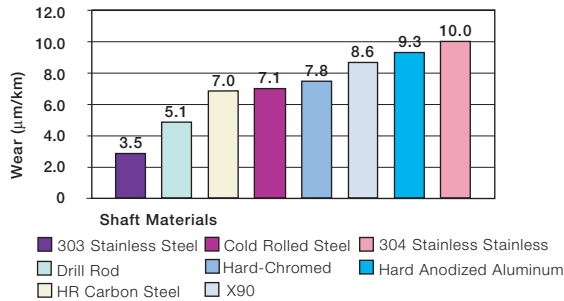
Graph 13.8: Wear of iglide® T500 with different shaft materials, p = 108 psi, v = 98 fpm
