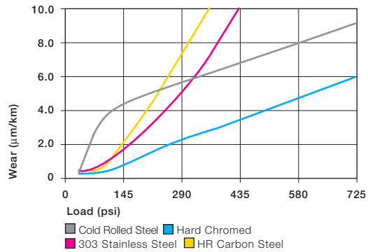
Graph 2.8: Wear of iglide® M250 with different shaft materials in rotational operation
