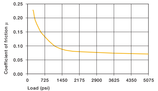
Graph 9.5: Coefficients of friction of iglide® P as a result of the load, v = 1.97 fpm
