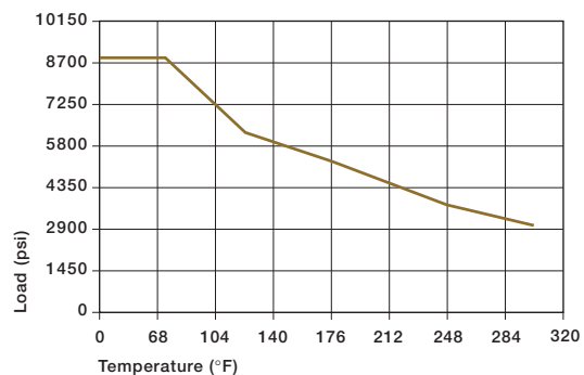
Graph 7.3: Recommended maximum permissible static surface pressure of iglide® L280 as a result of temperature
