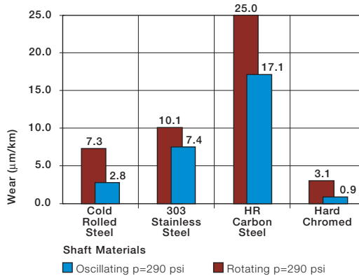
Graph 8.10: Wear for oscillating and rotating applications with different shaft materials at p = 290 psi
