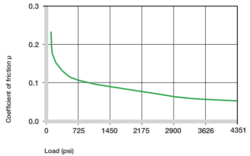
Graph 11.5: Coefficients of friction of iglide® A180 as a function of the load, v = 0.01 m/s
