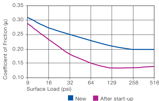
Graph 25.3: Coefficient of friction under load/DryLin® R, v = 29.5 fpm
