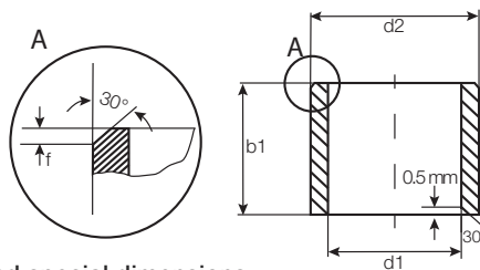
Dimensions according to ISO 3547-1 and special dimensions
