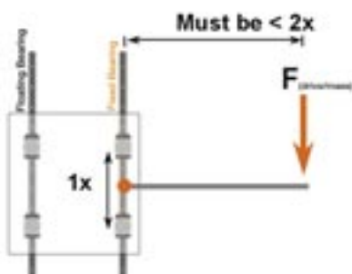
2:1 Rule = permissible distances of the applied forces
