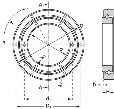
iglide® B180, PP cage, Glass Balls
