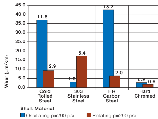
Graph 10.10: Wear for oscillating and rotating applications with different shaft materials p = 290 psi
