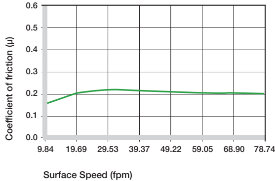
Graph 11.4: Coefficients of friction of iglide® A180 as a function of the running speed; p = 108 psi
