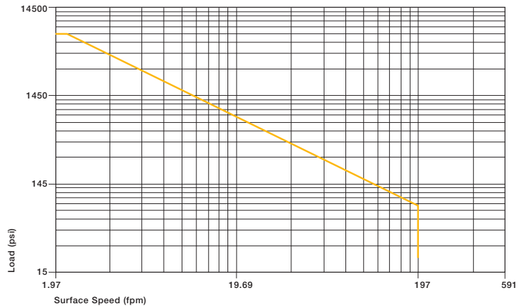
Graph 9.1: Permissible p x v value for iglide® P running dry against a steel shaft, at 68°F
