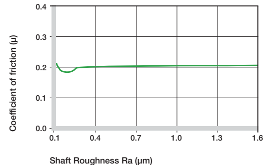
Graph 11.6: Coefficients of friction of iglide® A180 as a function of the shaft surface (shaft Cold Rolled Steel)
