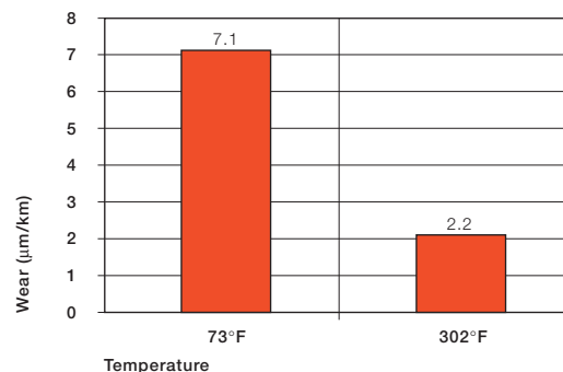
Graph 13.4: Wear of iglide® T500, Rotation with p = 108 psi, v = 98 fpm, shaft made of Cold Rolled Steel
