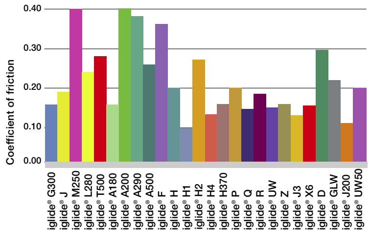
Coefficients of friction of the iglide® plain bearings for the recommended surface roughness and low load, p = 108.75 psi
