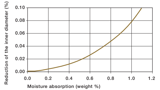
Graph 15.12: Effect of moisture absorption on iglide® Z plain bearings
