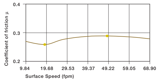
Graph 7.4: Coefficient of friction of iglide® L280 as a result of the surface speed, p = 108 psi, shaft made of Cold Rolled Steel
