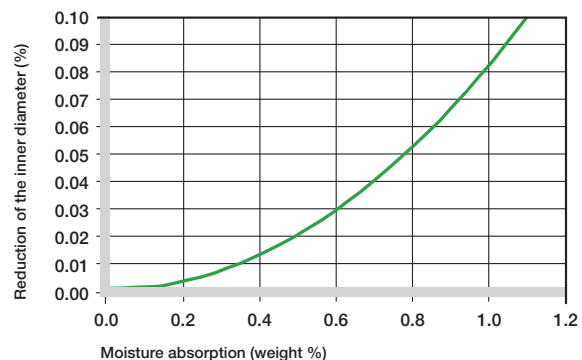
Graph 11.10: Effect of moisture absorption on iglide® A180 plain bearings
