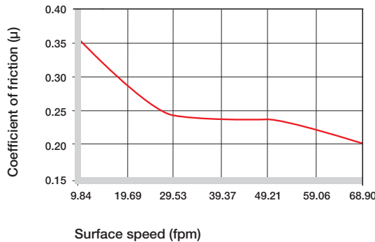
Graph 13.4: Coefficient of friction for iglide® X6 as a result of the running speed; p = 109 psi
