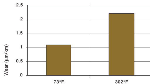
Graph 15.4: Wear of iglide® Z as a result of temperature, rotation with p = 108 psi, v = 98 fpm, (shaft Cold Rolled Steel)
