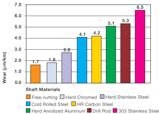
Graph 8.7: Wear of iglide® Q, rotating application with different shaft materials, p=108 psi, v=98 fpm
