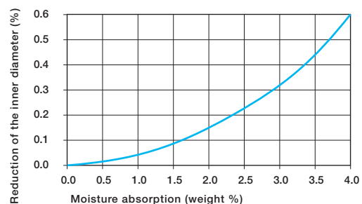
Graph 6.10: Effect of moisture absorption on iglide® G300 plain bearings
