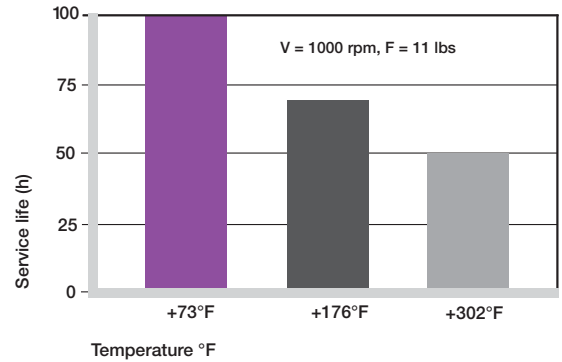
Service life of iglide® A500 plastic ball bearings at different ambient temperatures, dry
