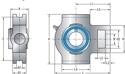
Main dimensions [mm]
