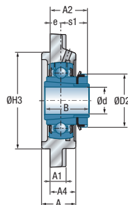
UKFS300H
