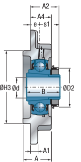
UKFC200H
