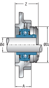
UCFC200CO(CC)
