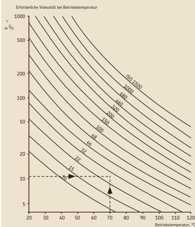
Fig. 2.6 Lubricant viscosity v vs. temperature t
