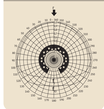
Fig. 3.6 Factors f_l and f_{l0} influence of the direction of load for LBHT linear ball bearings
