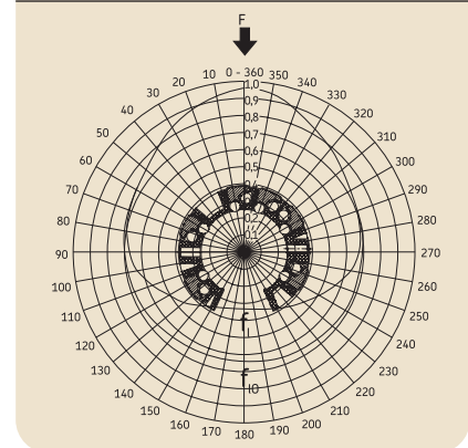
Fig. 3.5 Factor f_l and f_{l0} influence of the direction of load for LBCT and LBCF linear ball bearings
