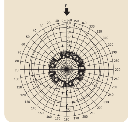
Fig. 3.4 Factor f_l and f_{l0} influence of the direction of load for LBCR and LBCD linear ball bearings
