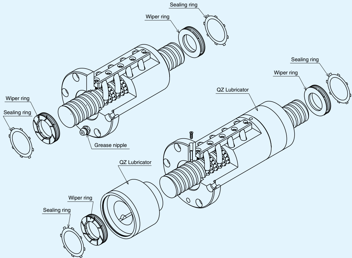
Fig. 2. Structural Drawings of QZ Lubricator and Wiper Ring
