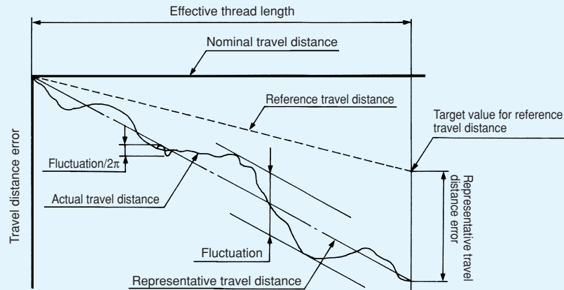
Fig. 1. Technical Terms on Travel Distance
